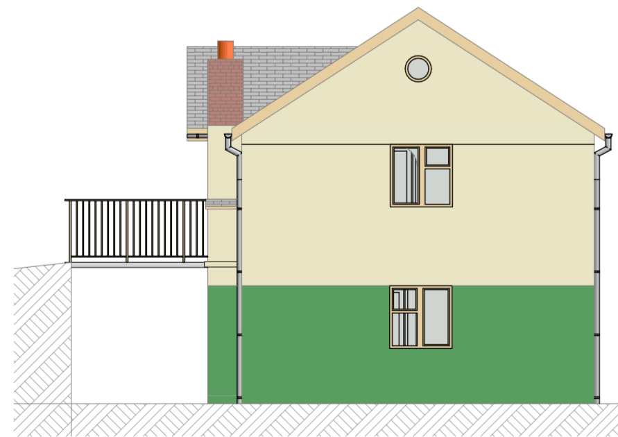
3 West Elevation 1:100
