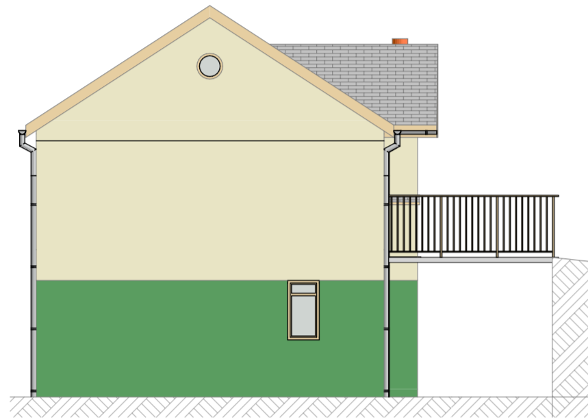
1 East Elevation 1:100
