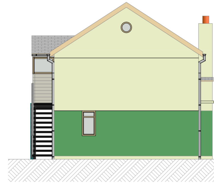
3 West Elevation 1:100
