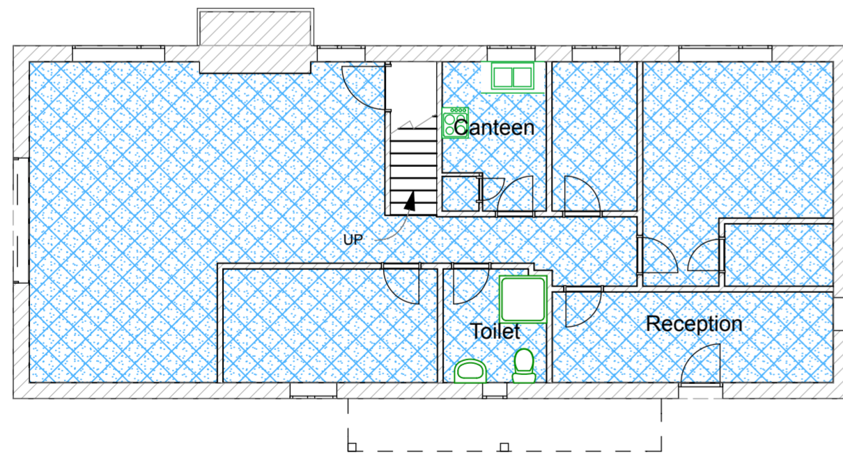
5 Ground Floor 1:100
